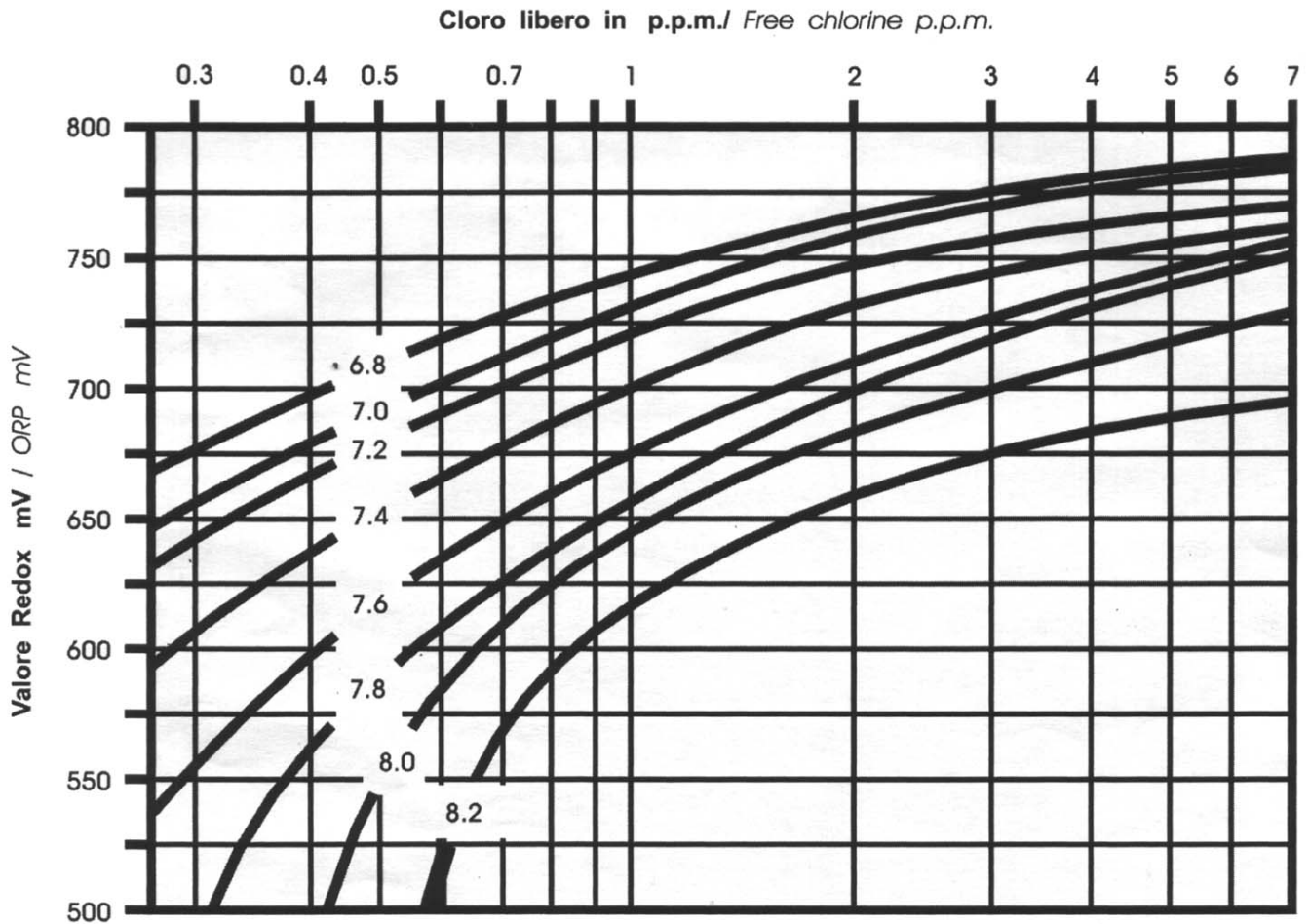
Curve pH / pH control curves
